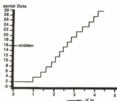
Fig. 2 S-meter curve IC-02E.
